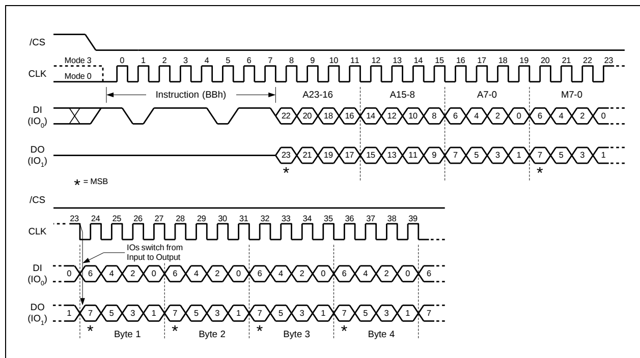
Figure 22a. Fast Read Dual I/O Instruction (Initial instruction or previous M5-4 \neq 10, SPI Mode only)
